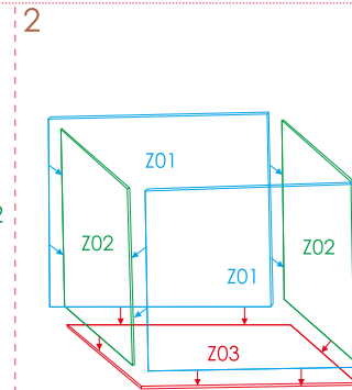
stick five pieces of plexiglass dust cover as shown
